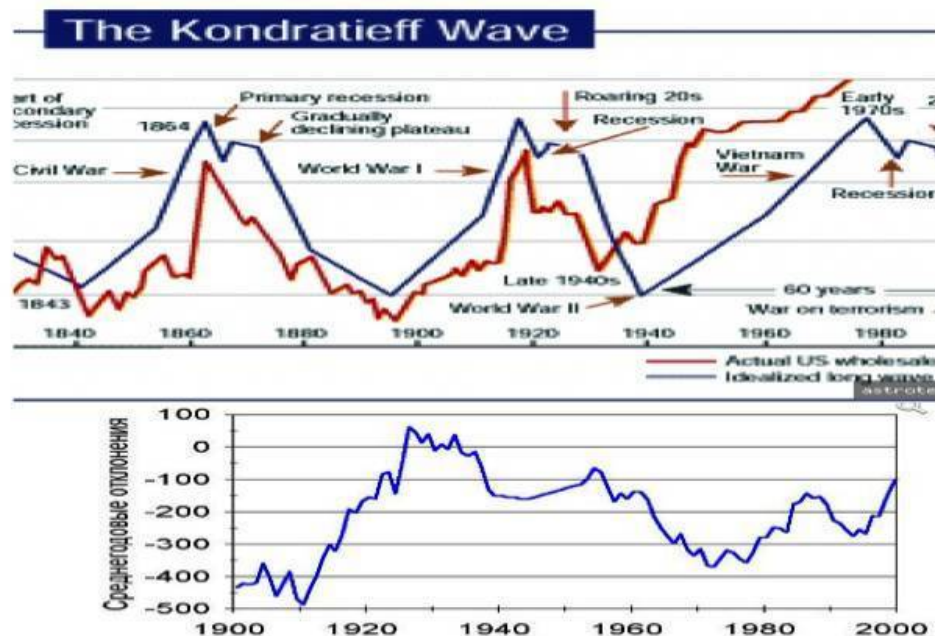
The Earth's angular rotational velocity and Kondratieff cycles with the displacement in 30 years
