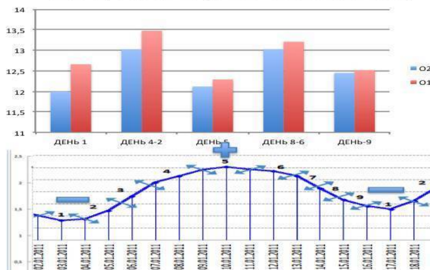
Data visualization of the connection between the EEG of surveyed depending on the day of cycle of changes in the Earth's rotational velocity
