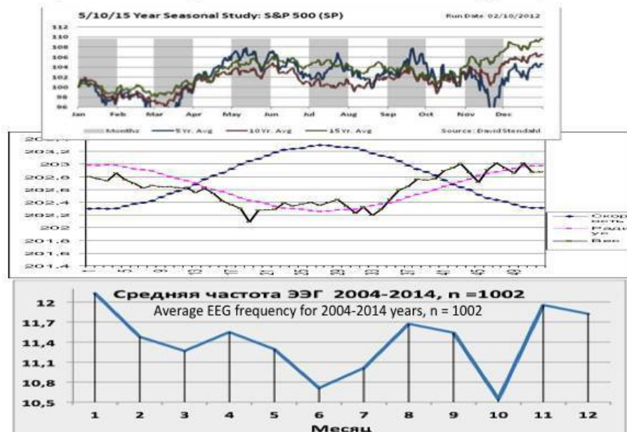
Annual cycles of the S&P 500 index change, the Earth's rotational velocity and EEG frequencies of surveyed in different months for the many years period
